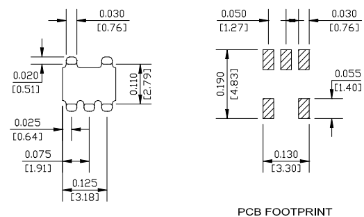
PCB FOOTPRINT
