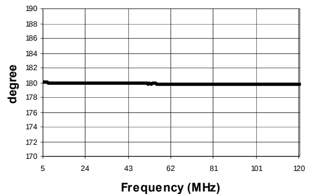
Phase Balance
