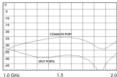
Return Loss (dB)
