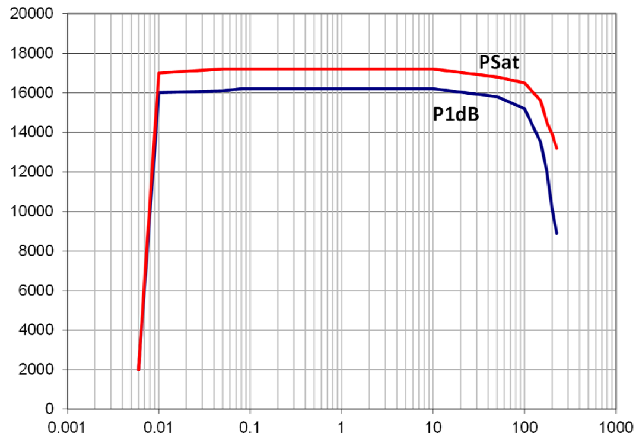
MODEL 16000A225A-A TYPICAL POWER OUTPUT
