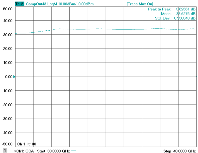
Figure 1-1: ERZ-HPA-3000-4000-32-E Psat
