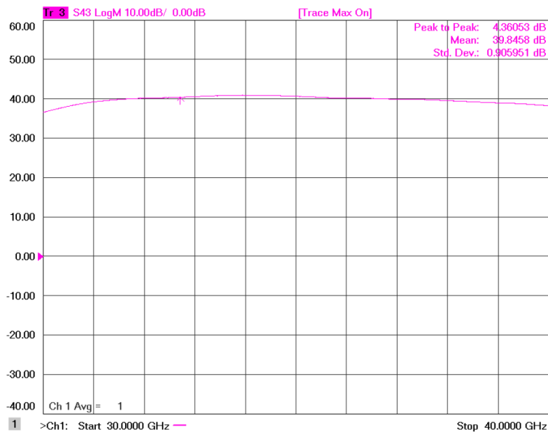
Figure 1-2: ERZ-HPA-3000-4000-32-E Small Signal Gain
