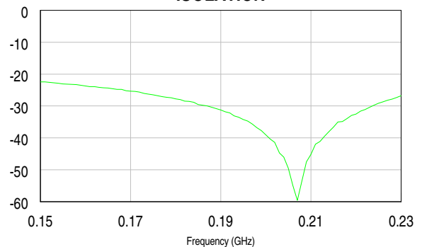
ISOLATION
