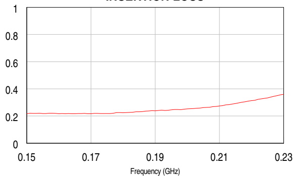
INSERTION LOSS
