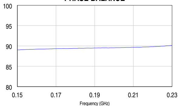
PHASE BALANCE
