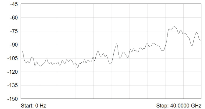
Typical Isolation (dB) Plot for 40GHz Terminated Versions
