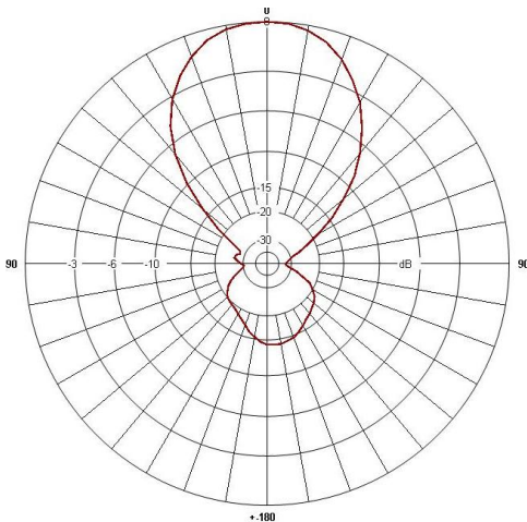
Elevation Pattern
