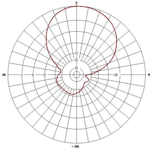
Elevation Pattern
