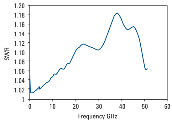
Typical SWR, 50 MHz to 50 GHz ( 25^{\circ}\text{C} \pm 10^{\circ}\text{C} ) for N8487A power sensor
