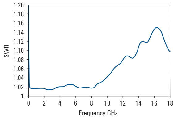
Typical SWR, 10 MHz to 18 GHz ( 25^{\circ}\text{C} \pm 10^{\circ}\text{C} ) for N8481A sensor
