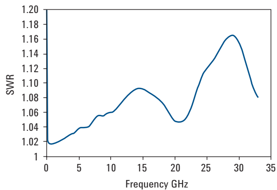
Typical SWR, 10 MHz to 26.5 GHz ( 25^{\circ}\text{C} \pm 10^{\circ}\text{C} ) for N8485A sensor
