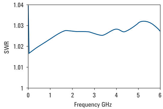
Typical SWR, 100 kHz to 6 GHz ( 25^{\circ}\text{C} \pm 10^{\circ}\text{C} ) for N8482A sensor
