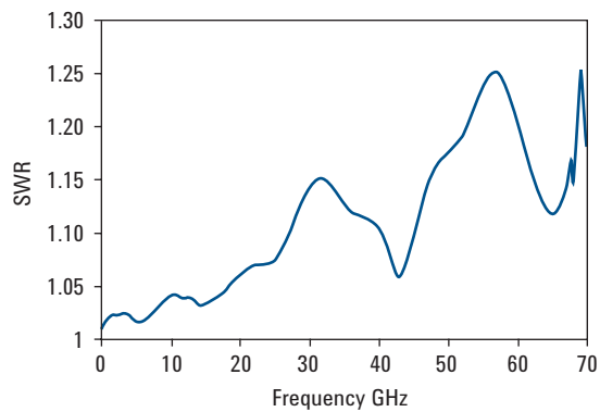
Typical SWR, 10 MHz to 70 GHz ( 25^{\circ}\text{C} \pm 10^{\circ}\text{C} ) for N8488A power sensor
