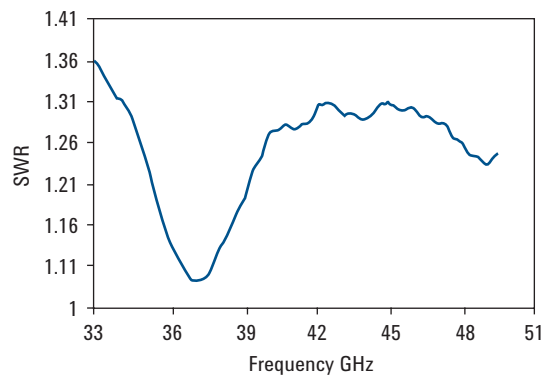
Typical SWR, 33 to 50 GHz ( 25^{\circ}\text{C} \pm 10^{\circ}\text{C} ) for N8486AQ power sensor
