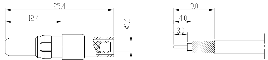
剥线尺寸 stripping dimension
