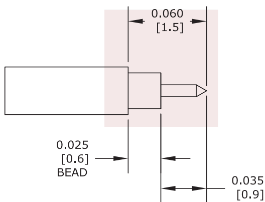
STRIPPING DIMENSIONS
