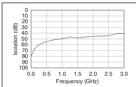
Figure 4. Typical Isolation
