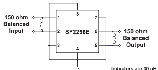
SF2256E Test Circuit
