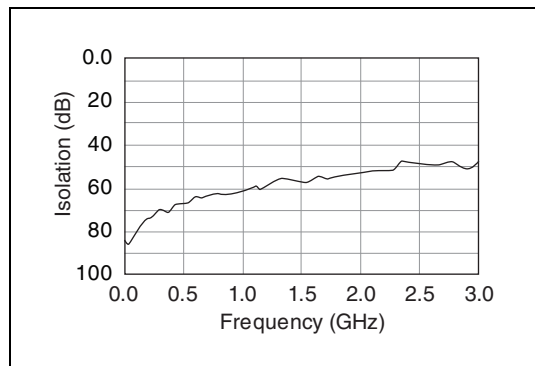
Figure 4. Typical Isolation
