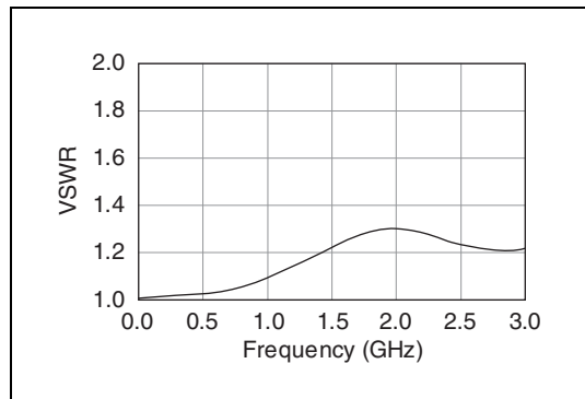
Figure 3. Typical Termination VSWR
