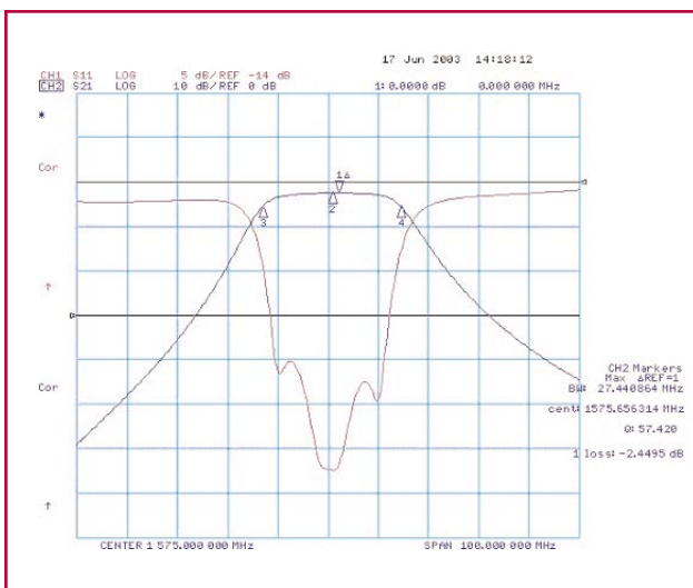
Amplitude Response
