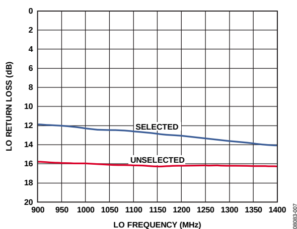
Figure 28. LO Return Loss, Selected and Unselected
