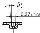
B-B Section
