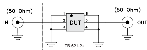
Fig 1. Block diagram of Test Circuit used for characterization, Test board TB-621-2+ Conditions: Attenuation, VSWR: Pin=-10 dBm
