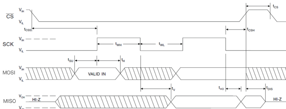
Figure 7-3: SPI timing
