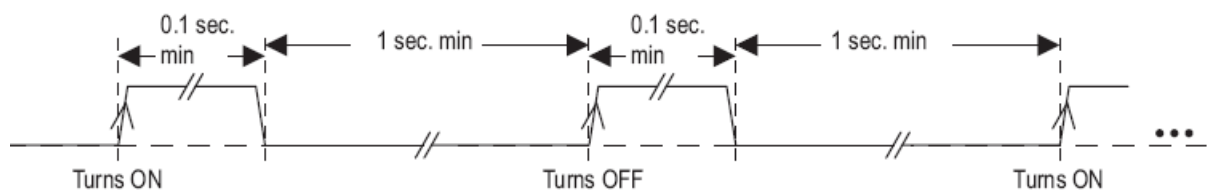
Figure 7-1: ON_OFF timing
