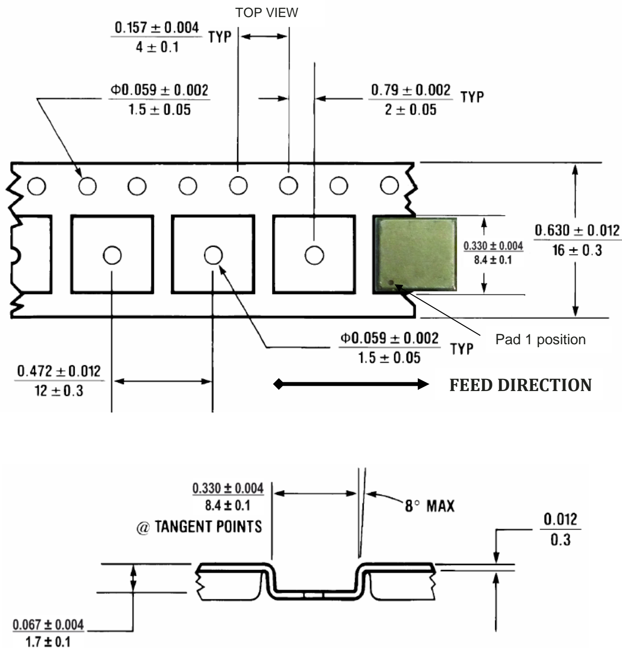
Figure 11-1: Carrier \frac{\text{inch}}{\text{millimeter}}
