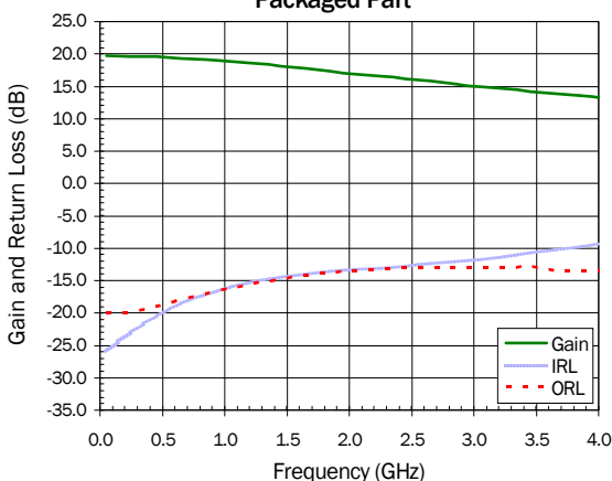
Gain and Return Loss - SGB2433Z
