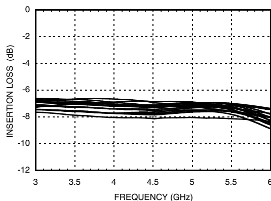
Insertion Loss vs. Temperature, Major States Only
