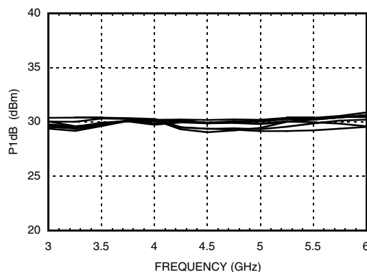
Input P1dB, Major States Only
