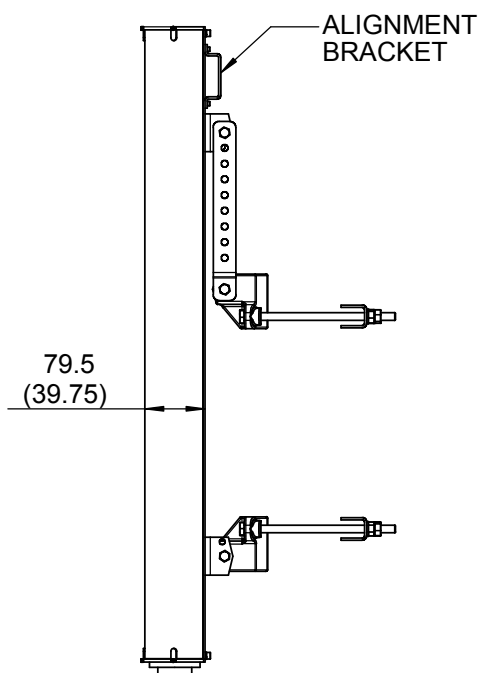
END VIEW
