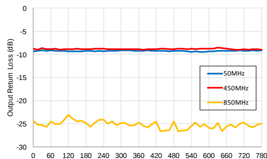
Temperature Range: Output Return Loss
