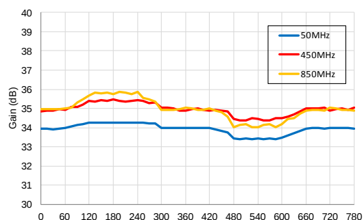
Temperature Range: Gain
