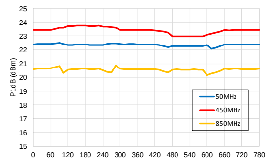
Temperature Range: P1dB
