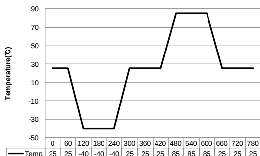
Temperature Cycle
