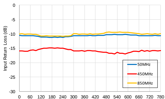
Temperature Range: Input Return Loss
