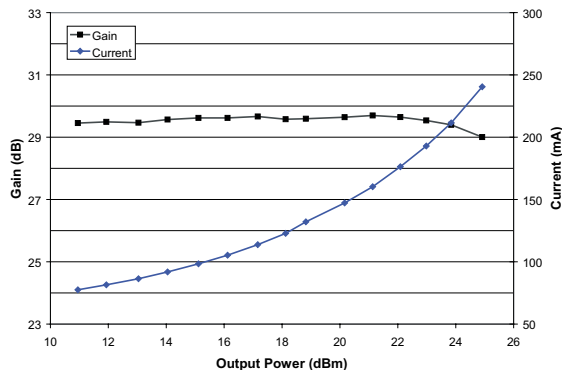
Figure 5: Gain and Current Consumption vs Output Power ( T_A = +25^\circ\text{C} , V_{CC} = +3.3\text{ V} , V_{REF} = +2.85\text{ V} , f = 2472\text{ MHz} , 54 Mbps 802.11g)
