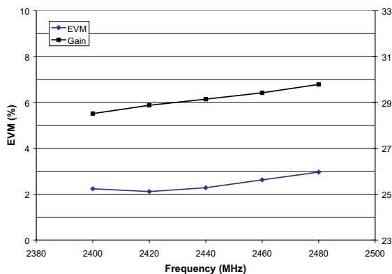
Figure 3: EVM and Gain vs Frequency ( T_A = +25^\circ\text{C} , V_{CC} = +3.3\text{ V} , V_{REF} = +2.85\text{ V} , P_{OUT} = +21\text{ dBm} , 54 Mbps 802.11g)
