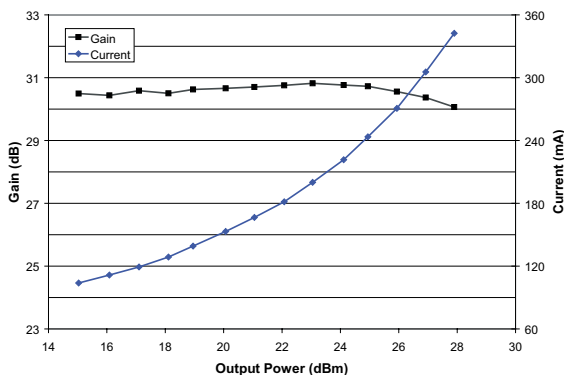
Figure 6: Gain and Current Consumption vs. Output Power ( T_A = +25^\circ\text{C} , V_{CC} = +5\text{ V} , V_{REF} = +2.85\text{ V} , f = 2472\text{ MHz} , 54 Mbps 802.11g)
