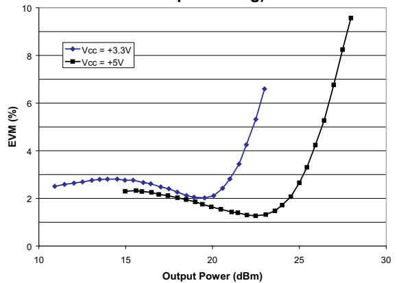
Figure 10: EVM vs. Output Power ( T_A = +25\text{ }^{\circ}\text{C} , V_{REF} = +2.85\text{ V} , f = 2472\text{ MHz} , 54 Mbps 802.11g)
