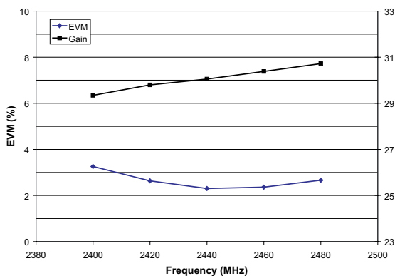
Figure 4: EVM and Gain vs Frequency ( T_A = +25^\circ\text{C} , V_{CC} = +5\text{ V} , V_{REF} = +2.85\text{ V} , P_{OUT} = +25\text{ dBm} , 54 Mbps 802.11g)
