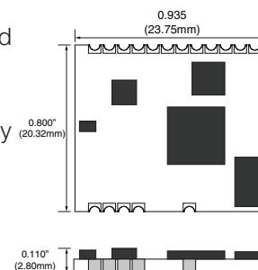
Figure 1: Package Dimensions
