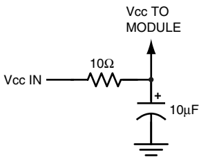
Figure 74: Supply Filter
