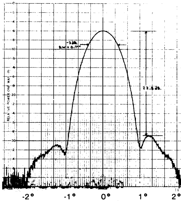
E-Plane — W-Band (12" Dia.)
