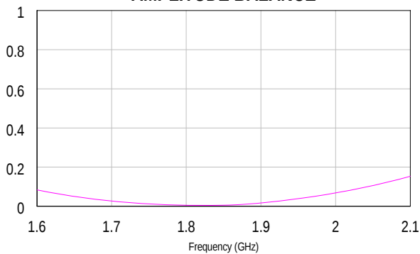
AMPLITUDE BALANCE
