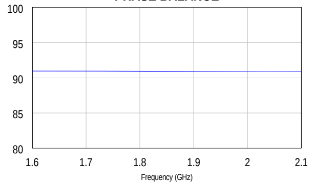
PHASE BALANCE
