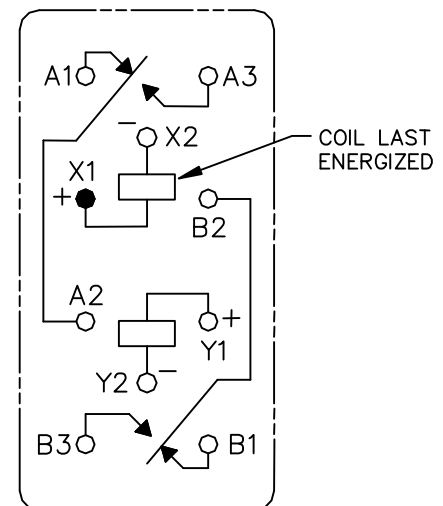
Figure 2 Terminal Locations and Circuit Diagram (bottom view)
