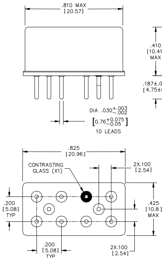
Figure 1 Outline dimensions
