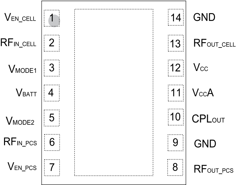
Figure 2: Pinout
