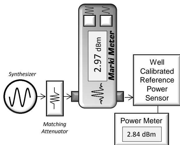
Fig. 6. Experimental Setup to Measure Accuracy
