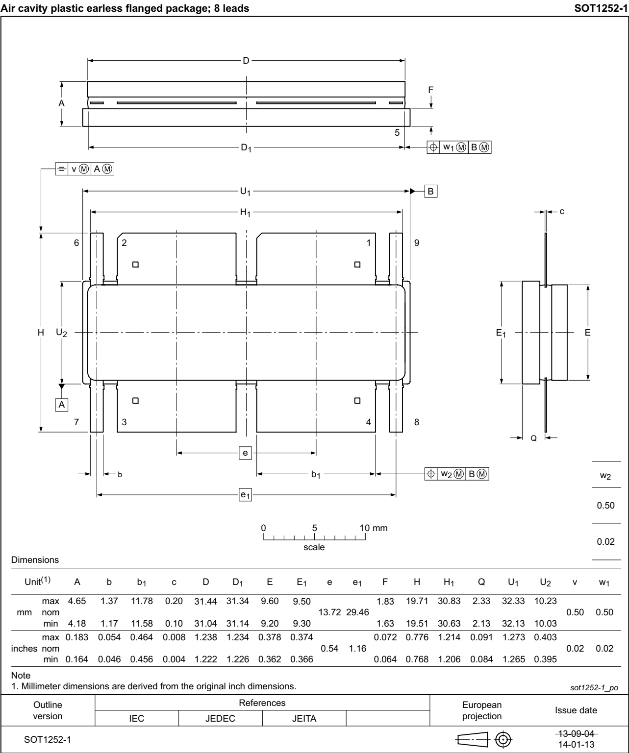
Fig 7. Package outline SOT1252-1
