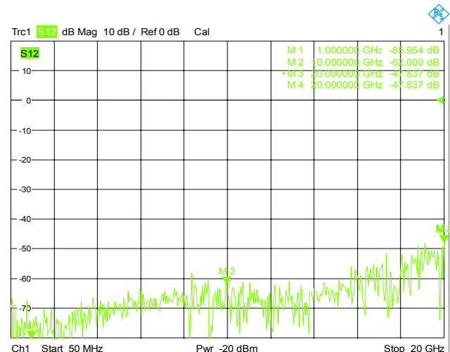
Amplifier Isolation (S12)
