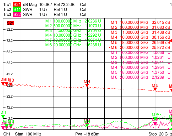
GAIN & VSWR (Over Frequency)
