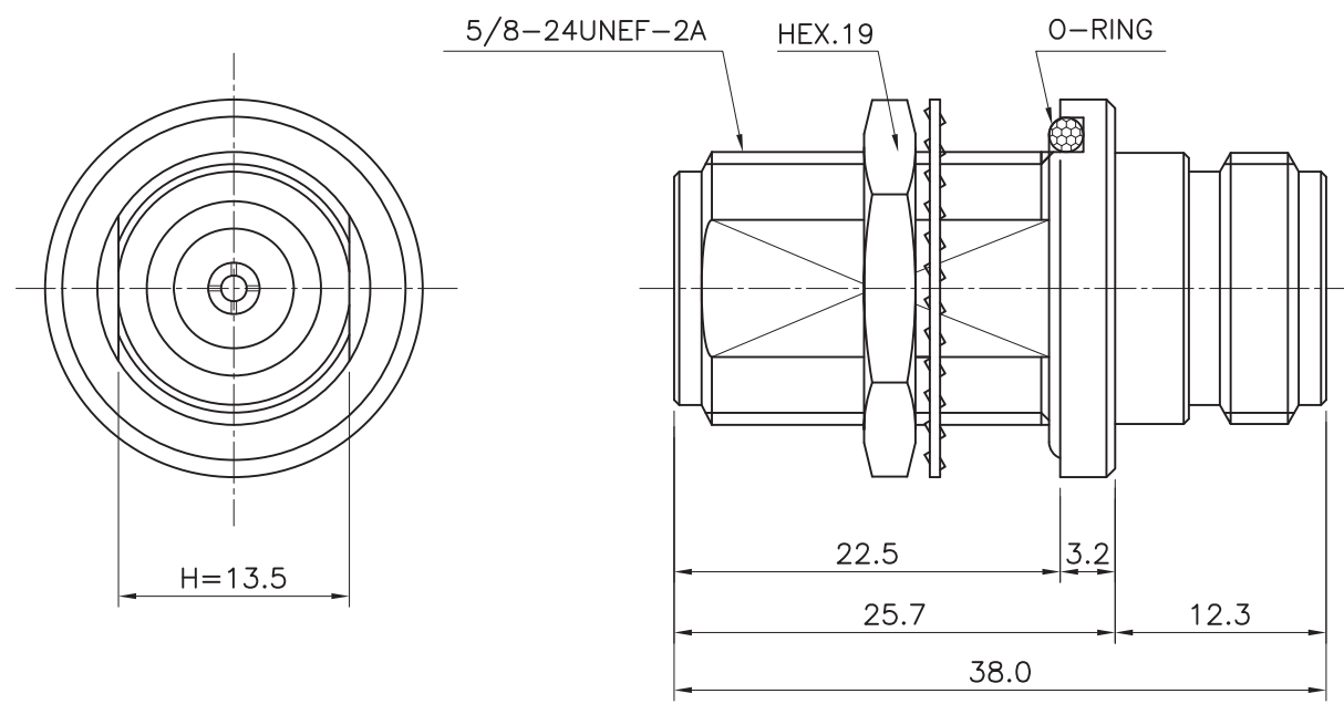
N-TYPE BULKHEAD JACK ADAPTOR with Panel seal
