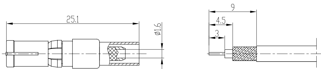
剥线尺寸 stripping dimension
