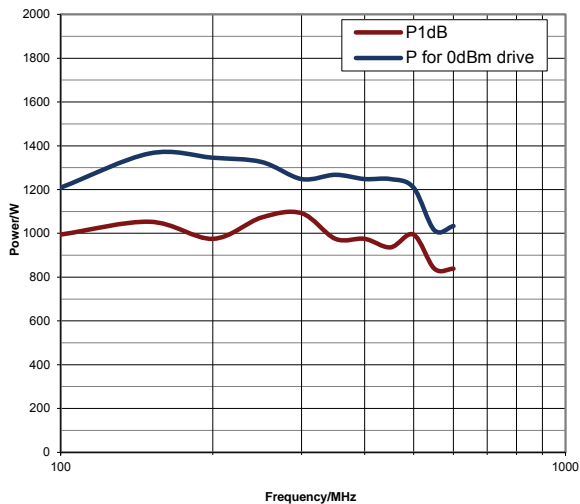
Typical peak envelope power plots
