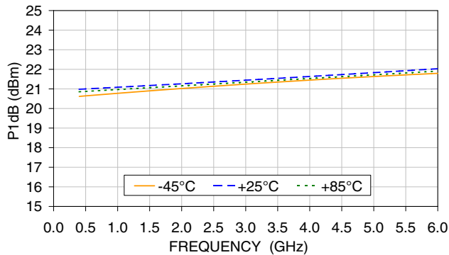
P1dB vs FREQUENCY & TEMPERATURE (1,4) @ VDS=4V, IDS=60mA
