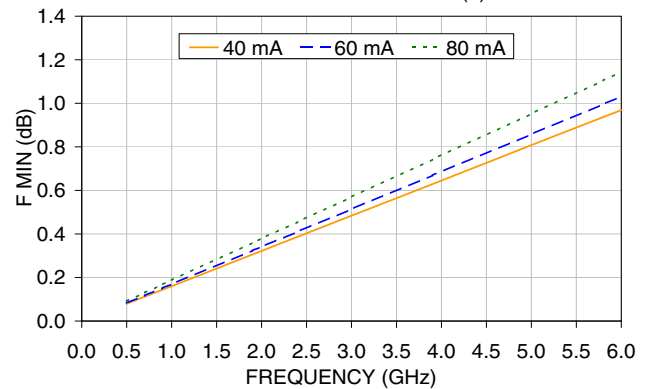
F Min vs FREQ @ VDS=3V (3)
