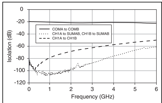
Figure 4. Typical Isolation
