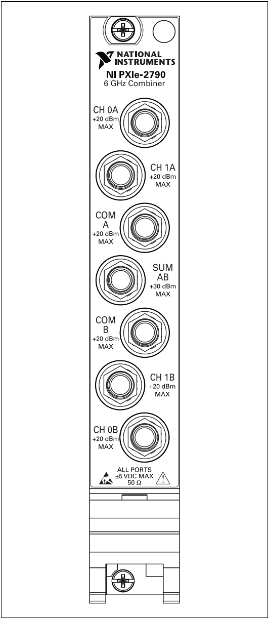
Figure 6. NI PXIe-2790 Front Panel Connector
