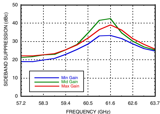
Figure 24. Sideband Suppression vs. Frequency and IF Gain
