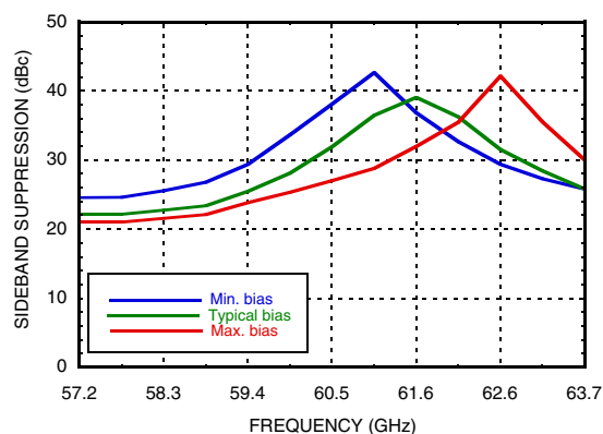
Figure 22. Sideband Suppression vs. Frequency across Voltage [2]
