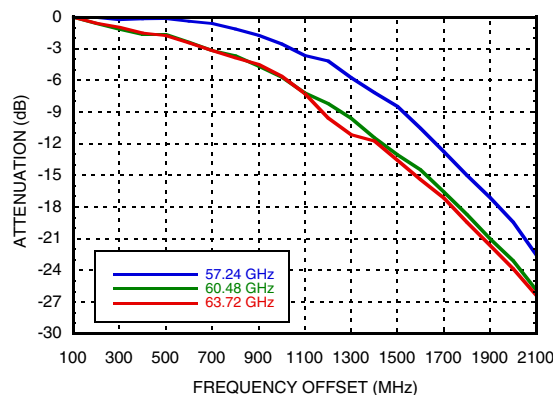
Figure 20. Single Sided Passband Response vs. Frequency [6]
