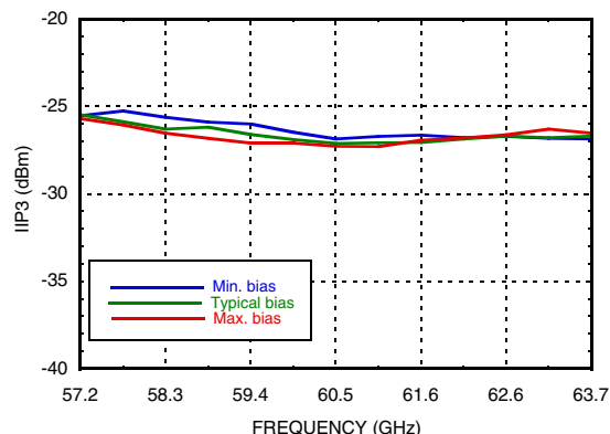
Figure 11. Input IP3 vs. Frequency Across Voltage [3][4]
