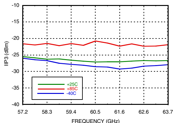
Figure 12. Input IP3 vs. Frequency Over Temperature [3][4]
