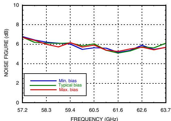
Figure 7. IC Noise Figure vs. Frequency Across Voltage [2][3]
