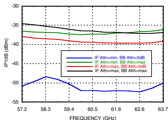
Figure 10. Input IP1dB vs. Frequency and Gain [3]
