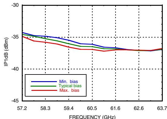
Figure 8. Input P1dB vs. Frequency Across Voltage [3][4]
