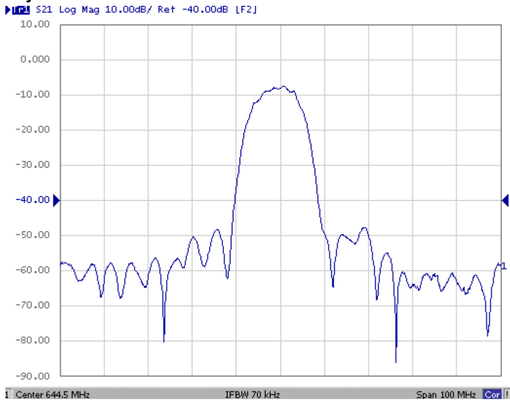
Fig-1 S21 Response Horizontal: 10MHz/Div
