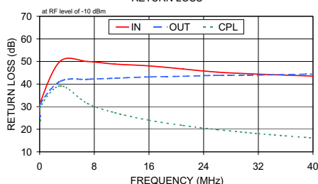
PDC-20-6-75 RETURN LOSS
