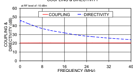
PDC-20-6-75 COUPLING & DIRECTIVITY
