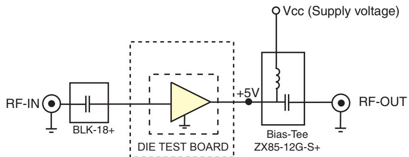
Figure 1: Block Diagram of Test Circuit used for characterization. Gain, Return loss, Output power at 1dB compression ( P_{1\text{ dB}} ), output IP3 (OIP3) and noise figure measured using Agilent's N5242A PNA-X microwave network analyzer.
