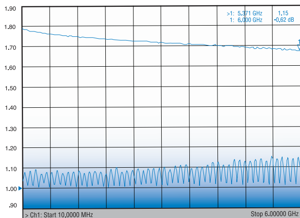
Typical VSWR (SPP-250-LLPL/NM/NM)
