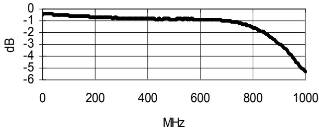
Insertion Loss
