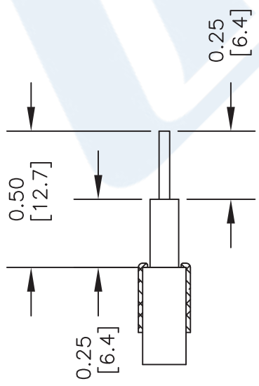
STRIPPING DIMENSIONS
