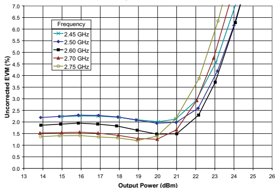
Figure 6: Uncorrected EVM vs. Output Power ( T_C = +25^\circ\text{C} , V_{CC} = +3.3\text{ V} , V_{BIAS} = +2.85\text{ V} , 54 Mbps OFDM Modulation, system EVM approx. 0.8 %)
