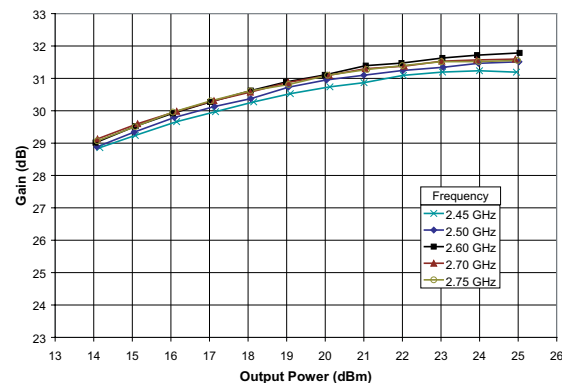
Figure 7: Gain vs. Output Power ( T_C = +25^\circ\text{C} , V_{CC} = +4.2\text{ V} , V_{BIAS} = +2.85\text{ V} , 54 Mbps OFDM Modulation)
