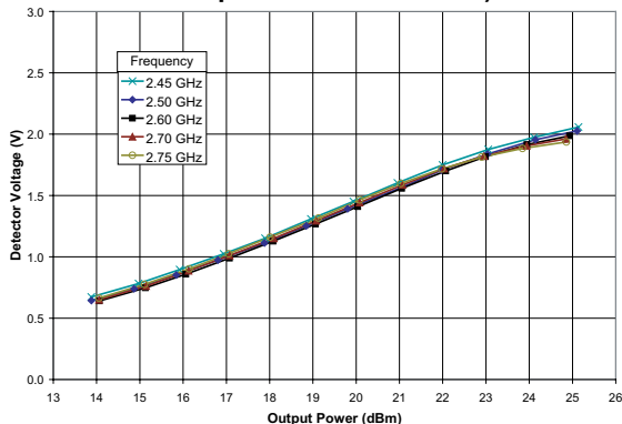
Figure 13: Detector Voltage vs. Output Power
