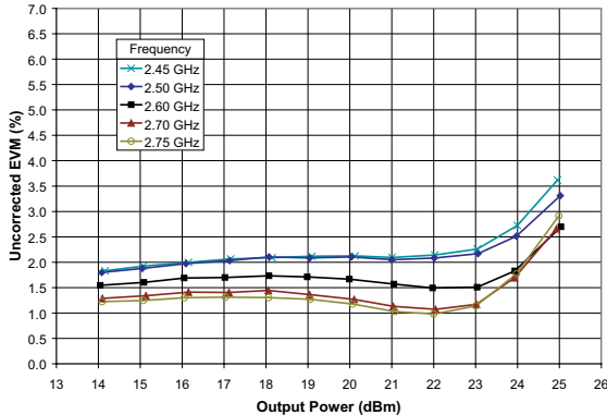
Figure 8: Uncorrected EVM vs. Output Power ( T_C = +25^\circ\text{C} , V_{CC} = +4.2\text{ V} , V_{BIAS} = +2.85\text{ V} , 54 Mbps OFDM Modulation, system EVM approx. 0.8 %)
