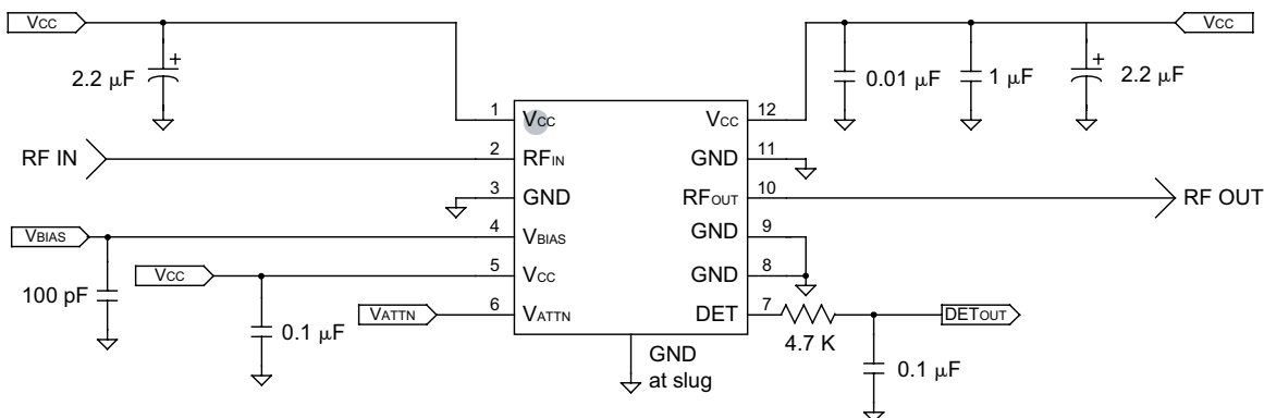
Figure 19: Application Circuit
