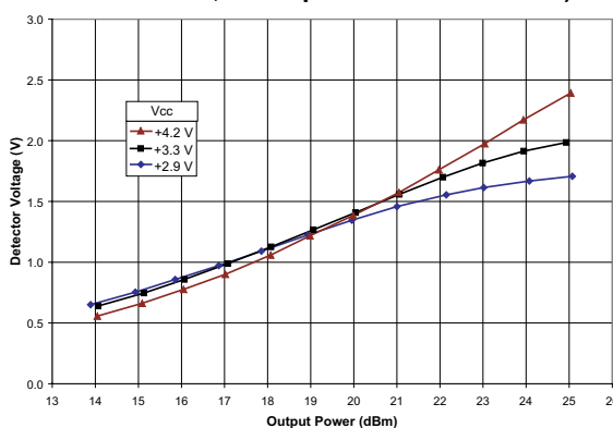
Figure 14: Effects of Supply Voltage ( V_{CC} ) on Detector Voltage
