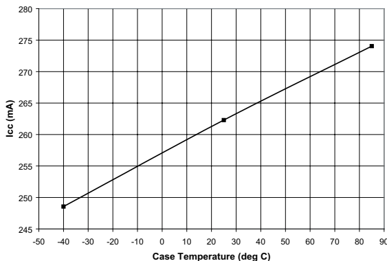
Figure 17: Supply Current vs. Case Temperature ( V_{CC} = +3.3 V, V_{BIAS} = +2.85 V, f = 2.6 GHz, P_{OUT} = +22 dBm, 54 Mbps OFDM Modulation)
