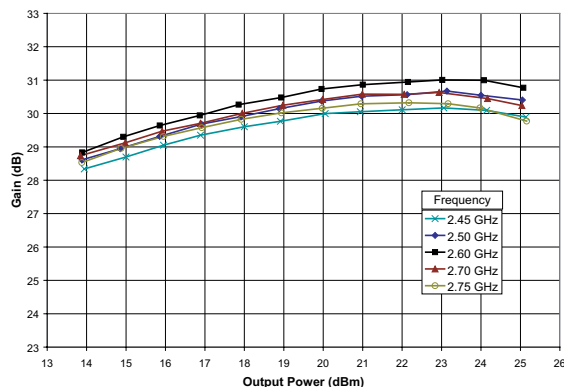
Figure 5: Gain vs. Output Power ( T_C = +25^\circ\text{C} , V_{CC} = +3.3\text{ V} , V_{BIAS} = +2.85\text{ V} , 54 Mbps OFDM Modulation)
