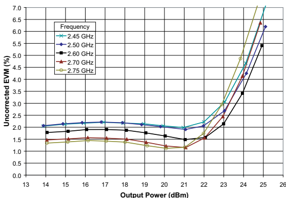
Figure 8: Uncorrected EVM vs. Output Power ( T_C = +25^\circ\text{C} , V_{CC} = +4.2\text{ V} , V_{BIAS} = +2.85\text{ V} , 54 Mbps OFDM Modulation, system EVM approx. 0.8 %)
