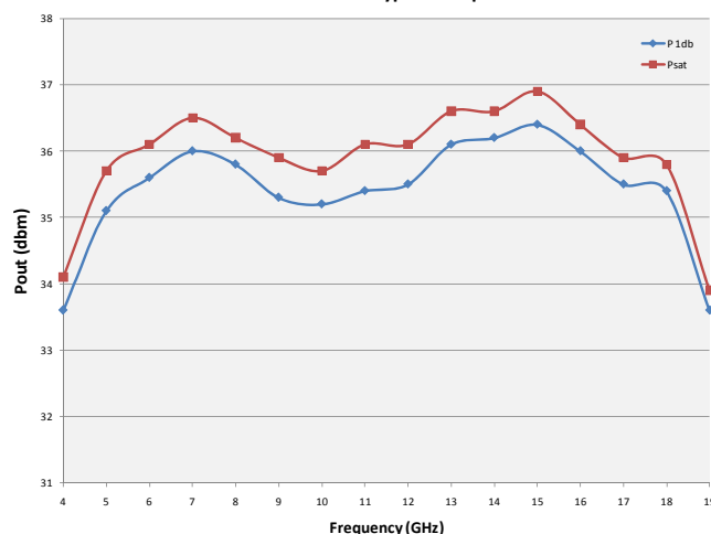
35HM4G18-22 Typical Output Power
