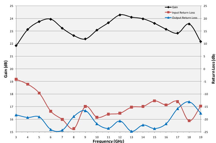
35HM4G18-22 Typical Gain & Return Loss
