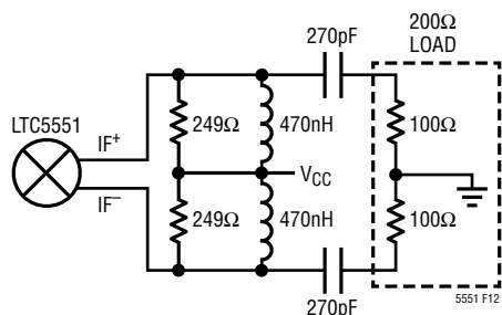
Figure 12. Wideband 200 \Omega Differential Output
