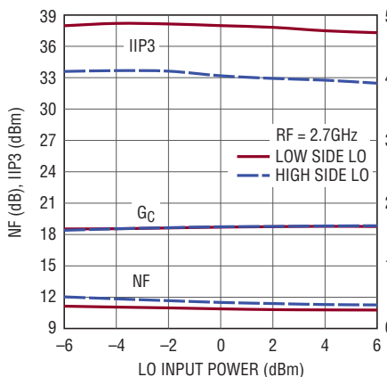
2.7GHz Conversion Gain, IIP3 and NF vs LO Power
