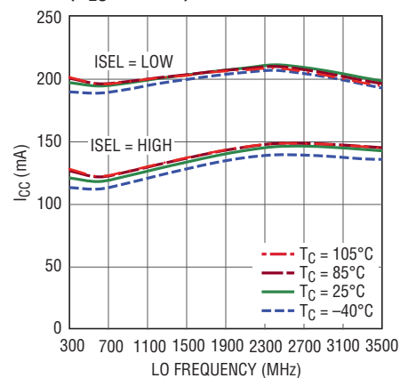
Supply Current vs LO Frequency ( P_{LO} = 0\text{dBm} )
