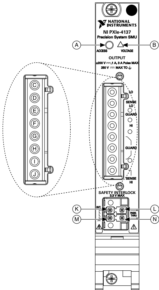
Figure 8. Front Panel
