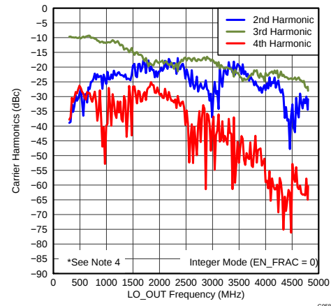
Figure 60. LO Harmonics
