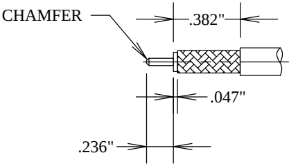
STRIPPING DIMENSIONS
