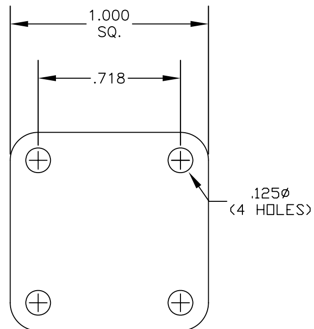
MOUNTING HOLES
